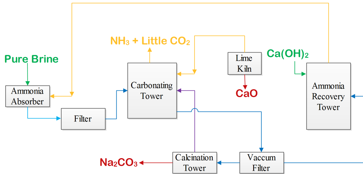
Figure: Manufacturing of Sodium Carbonate by Solvay's Process
